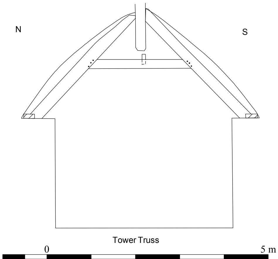
Figure 8: Tower and Central Range Trusses Scale 1:50
