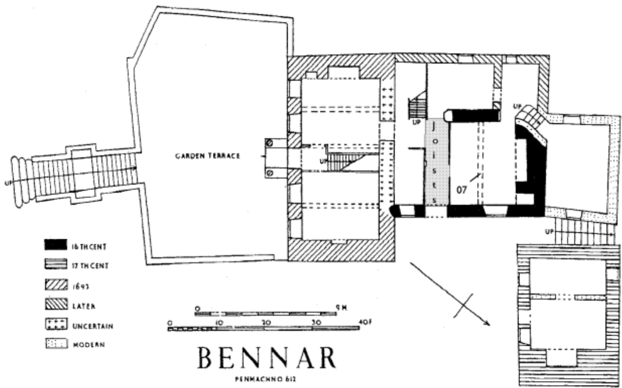
Figure 1: Plan showing the various parts of the building and the areas from which samples were taken for dendrochronology. Samples 03-06 came from the shaded area marked 'Joists' and the axial beam in the kitchen is shown as sample 07 . The truss sampled was above this axial beam. Adapted from an original in RCAHMW An Inventory of . . . Caernarvonshire, Volume I: East (1956).
