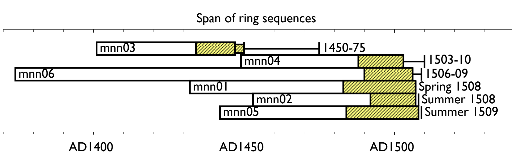
Figure 3: Bar diagram showing the relative positions of overlap of the dated series, along with their interpreted likely, or actual, felling date ranges. Hatched yellow sections represent sapwood rings, and narrow sections of bar represent additional unmeasured rings
