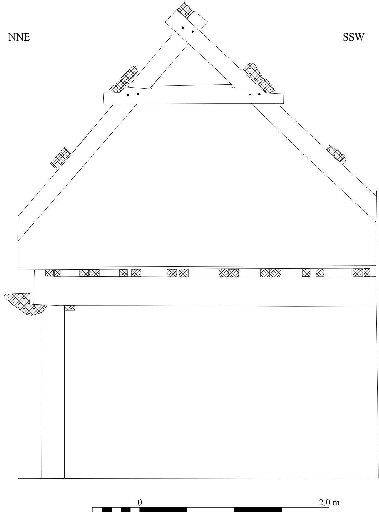
Figure 7: Truss 3 Scale 1:25
