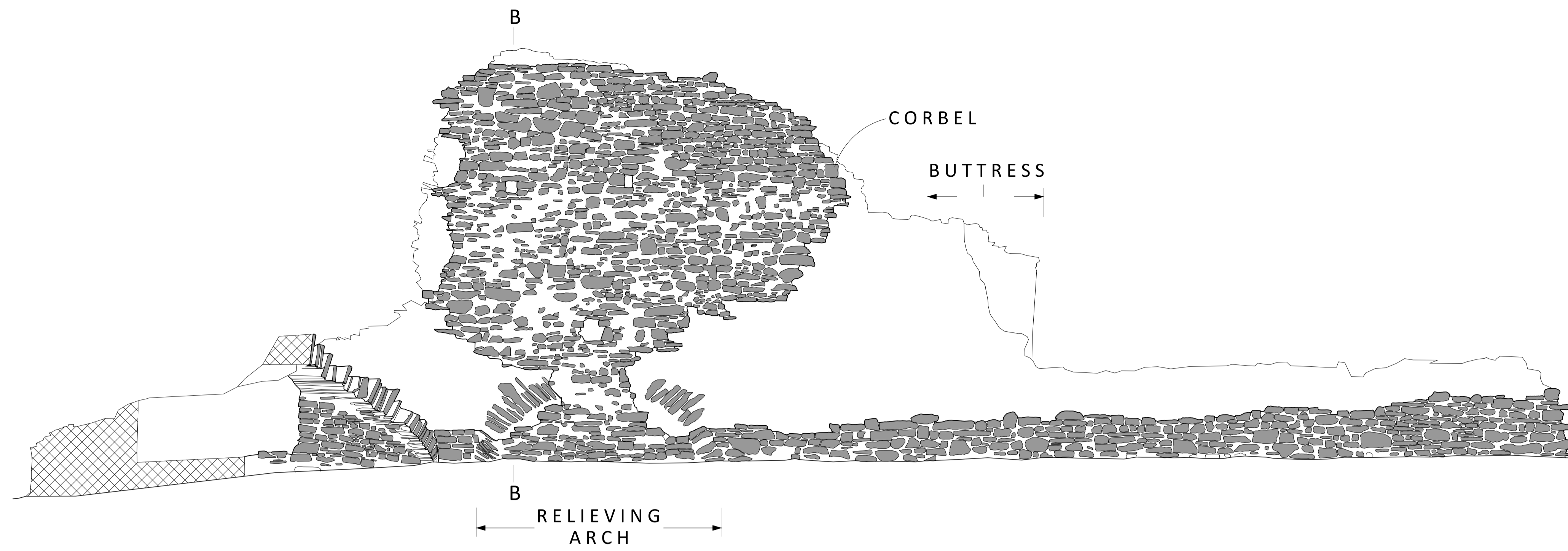
SOUTH INTERNAL ELEVATION
