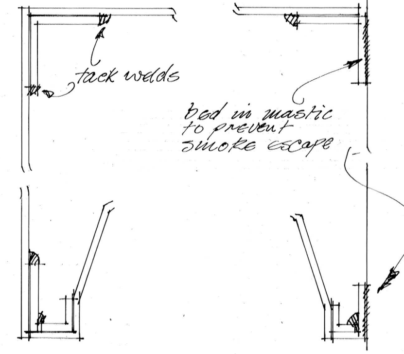
DETAIL OF METAL HOOD.
