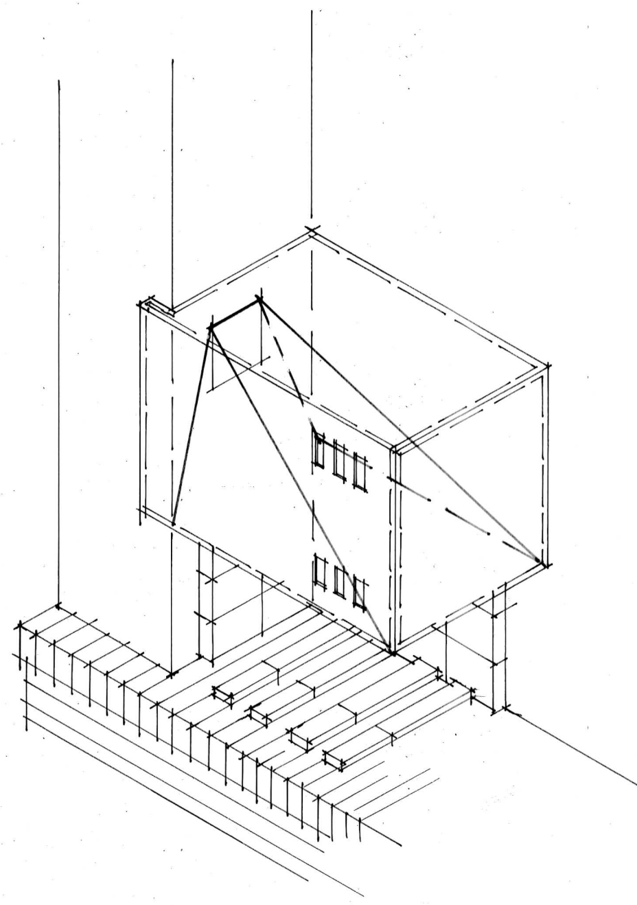
ISOMETRIC VIEW SHOWING POSITION OF INTERNAL HOOD TO FIREPLACE CANOPY
