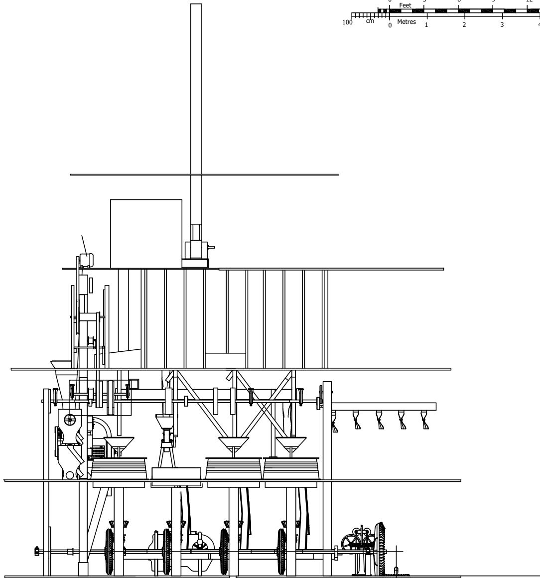
SIDE ELEVATION
