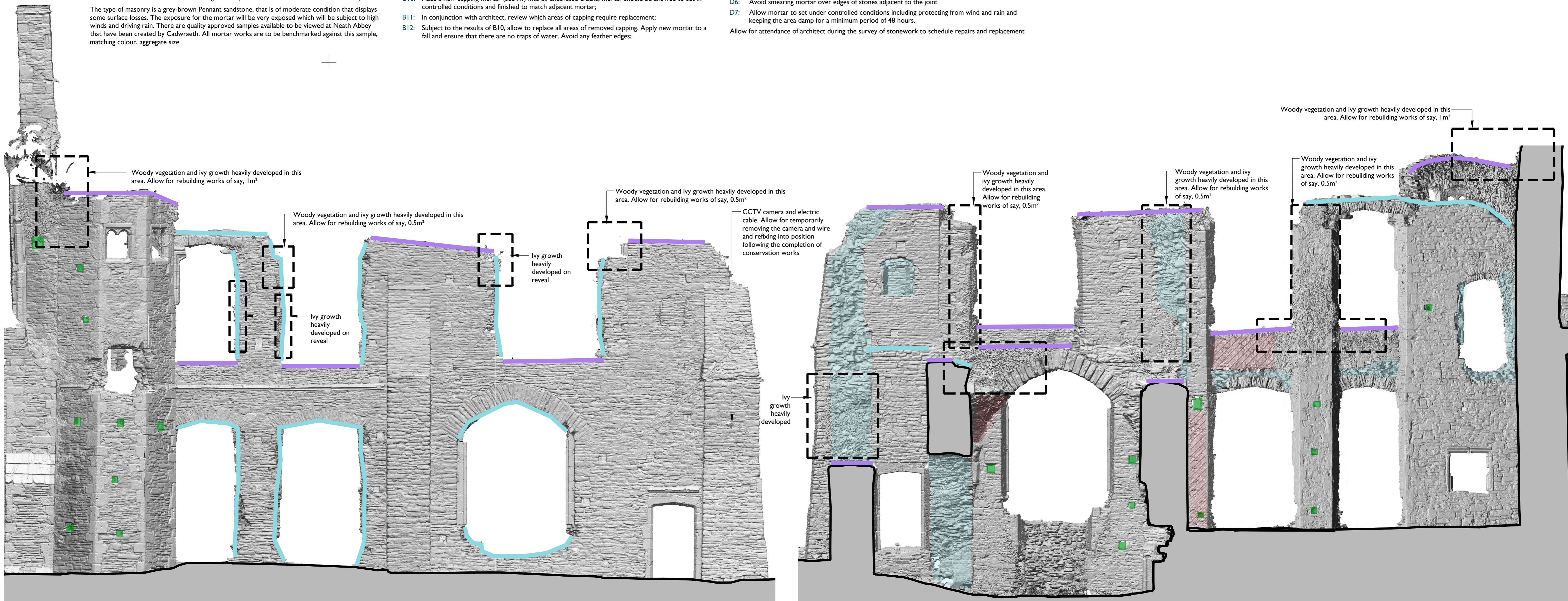
1 Elevation 1.1.1 (South face RHS) 210 1:50
