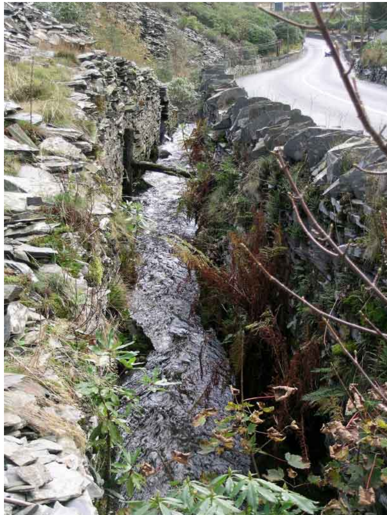
Plate 52 Site 6 Afon Barlwyd culvert, south end
