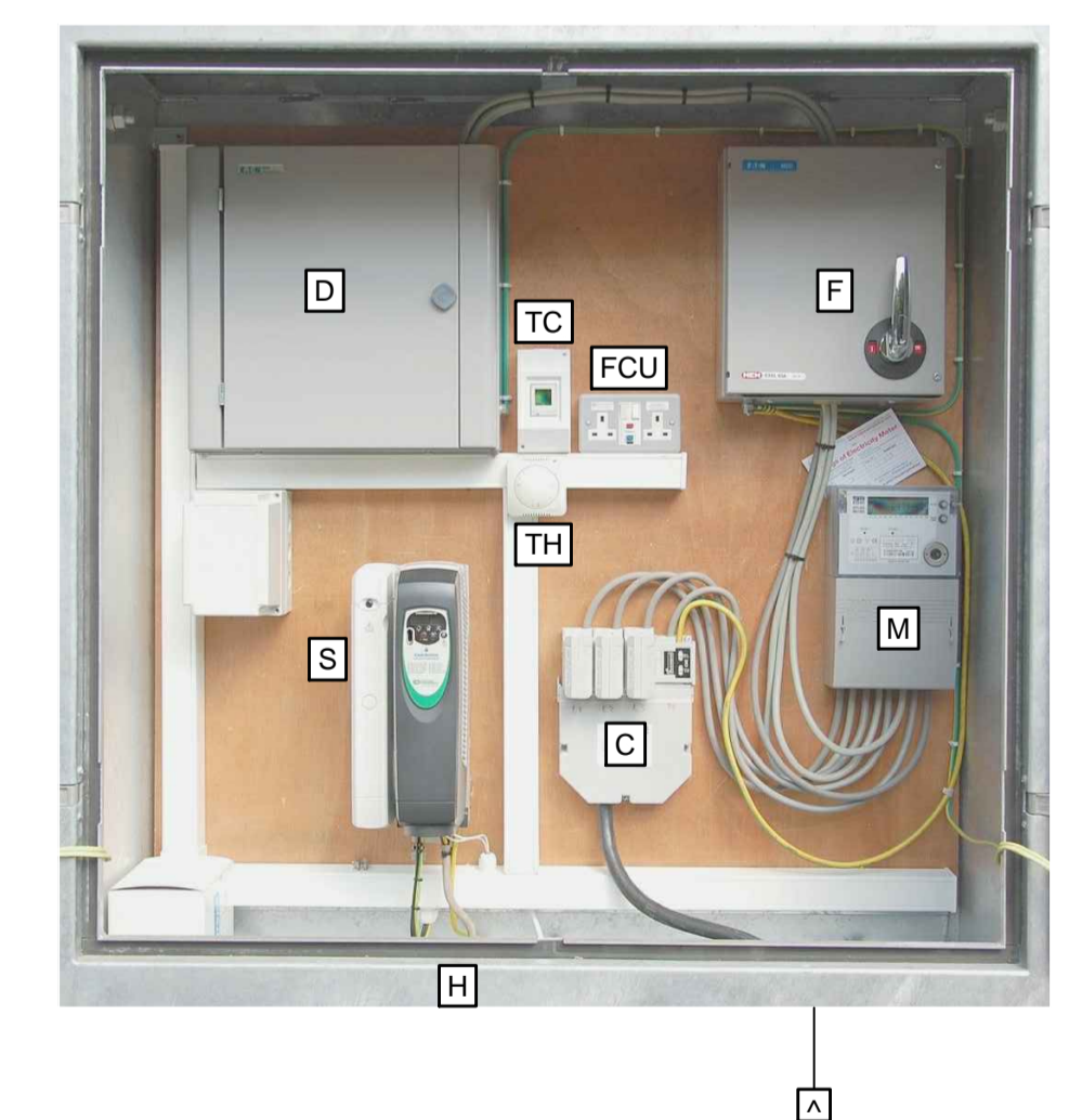
Detail E Electrical equipment and cabinet details | not to scale
