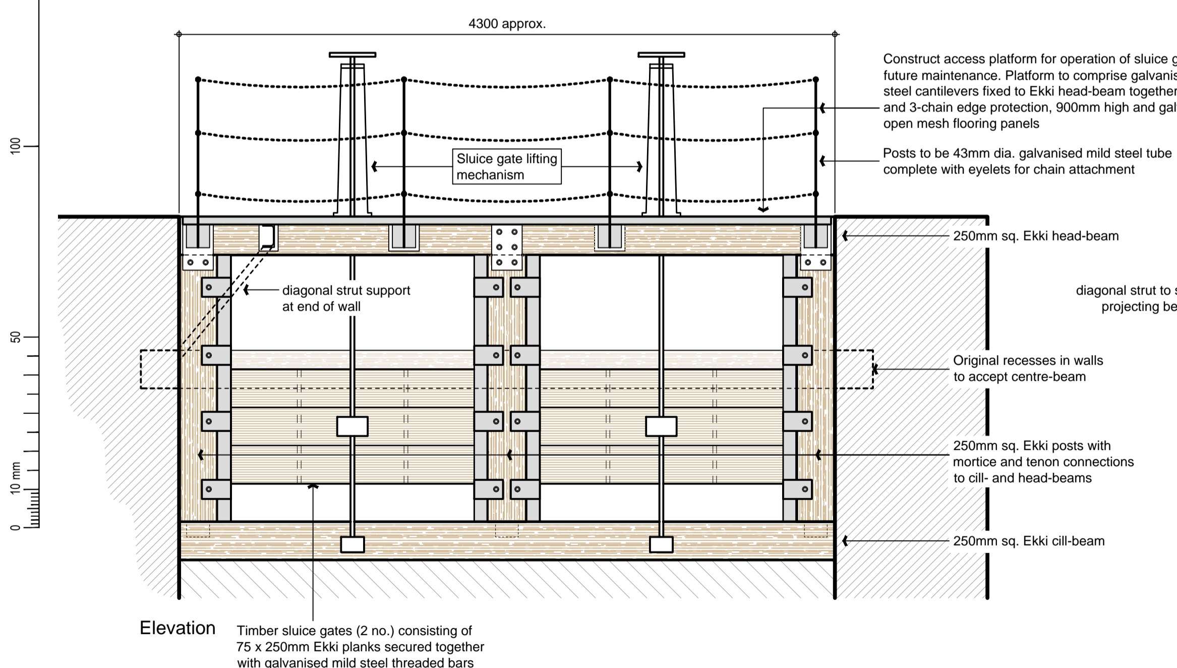
Detail B Replacement sluice gates, frame and mechanisms | scale 1:25
