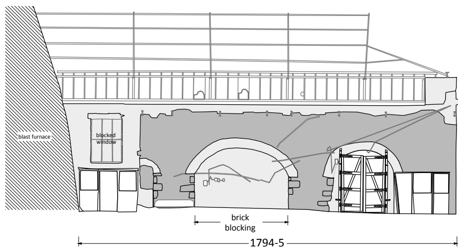
Front Wall Section B-B
