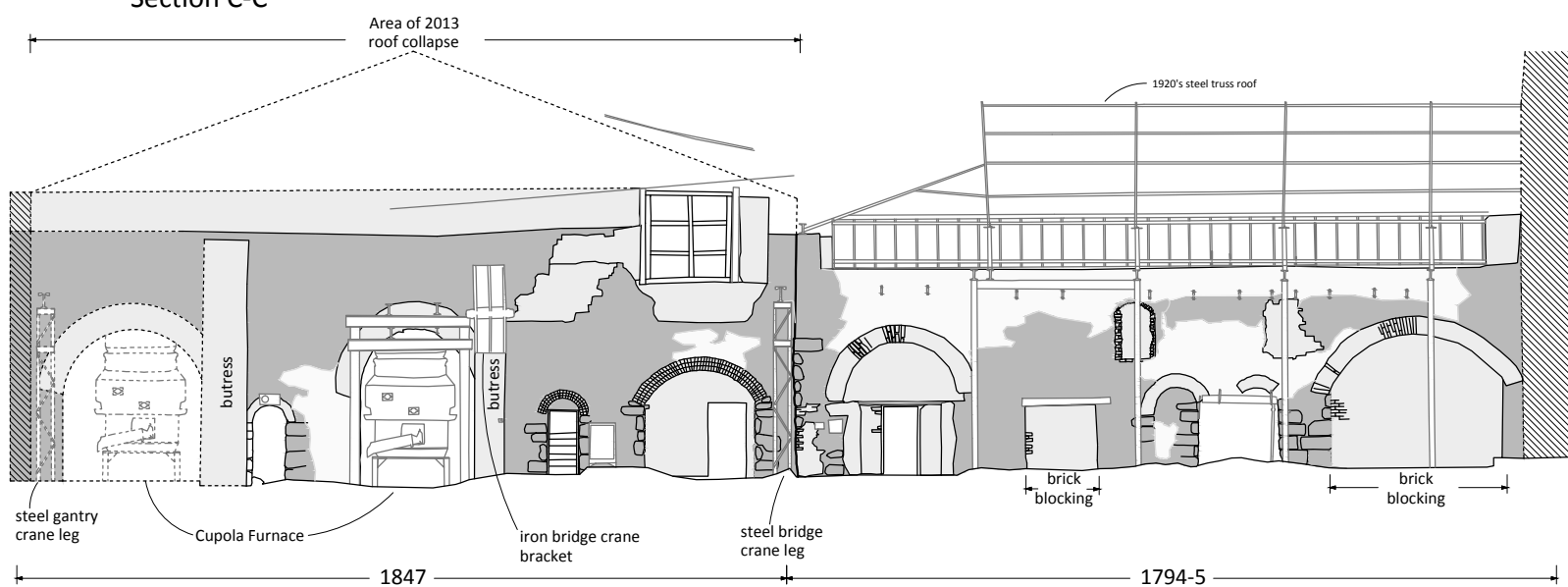
Rear Wall Section C-C
