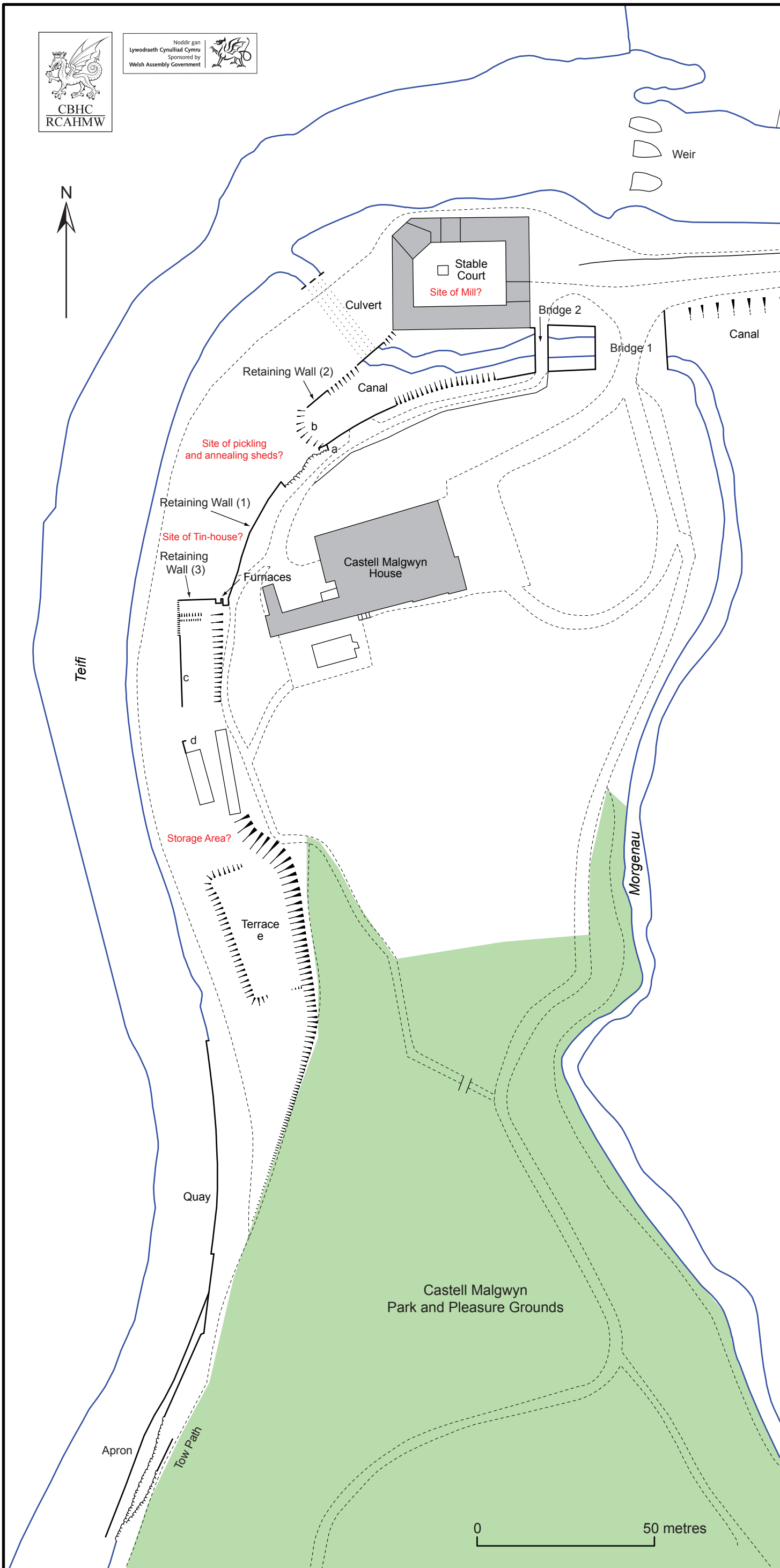
Fig 2: RCAHMW Survey and Interpretation plan showing surviving features of the Castell Malgwyn Tinplate Works
